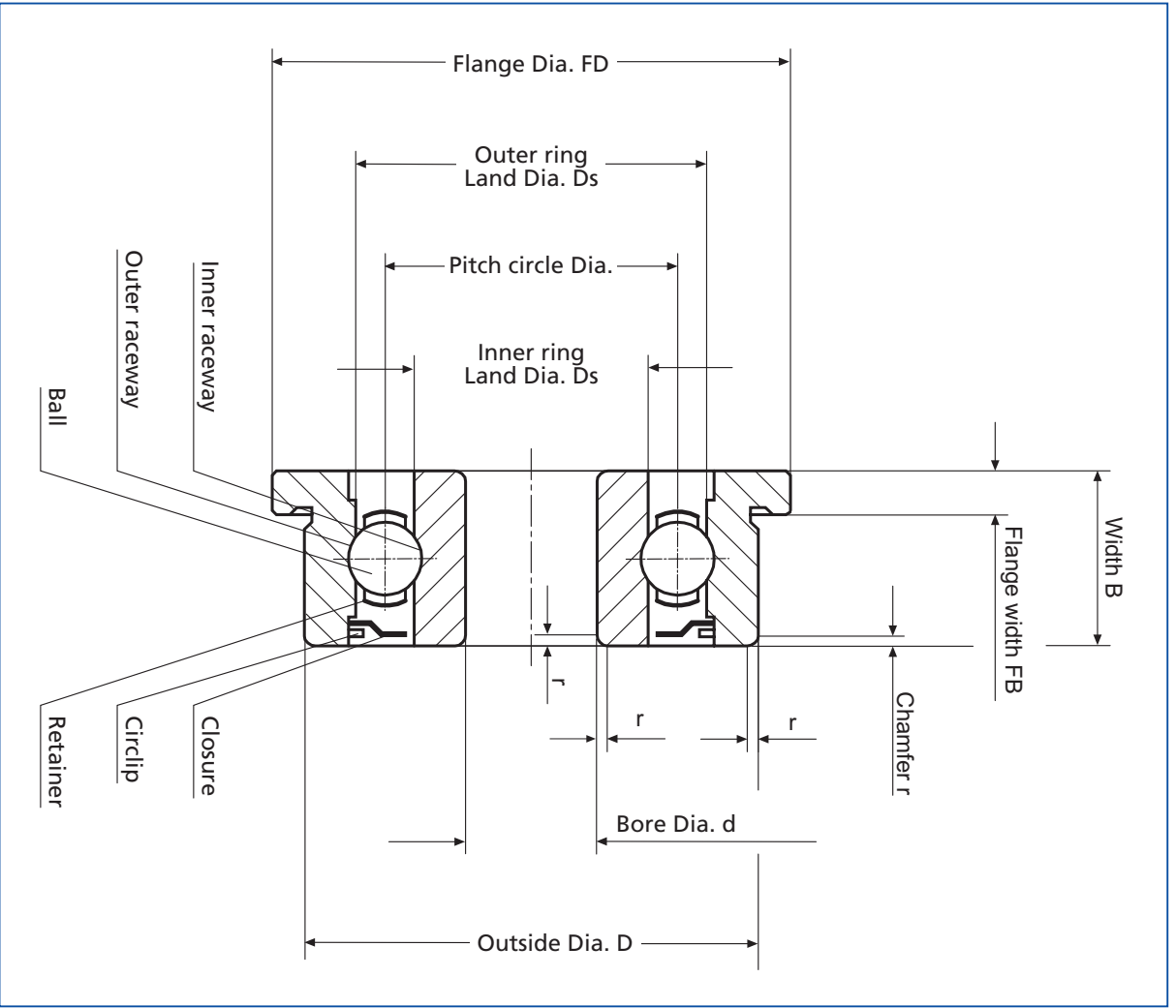
Fig. 28: Ball bearing parts
